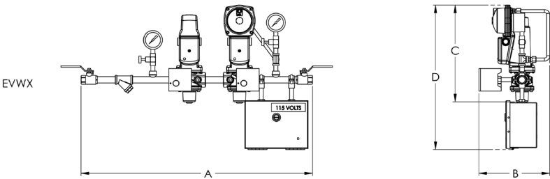
DIMENSIONS FOR EVWX PACKAGES
