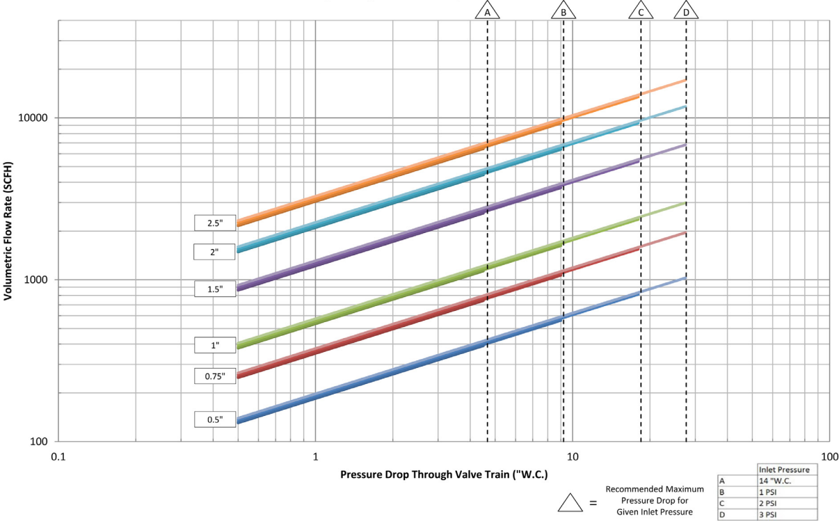
ETTER Valveworx Xtra - EVWX Low Inlet Pressure Capacity Chart - 1/2 PSI - 3 PSI Inlet Pressure
