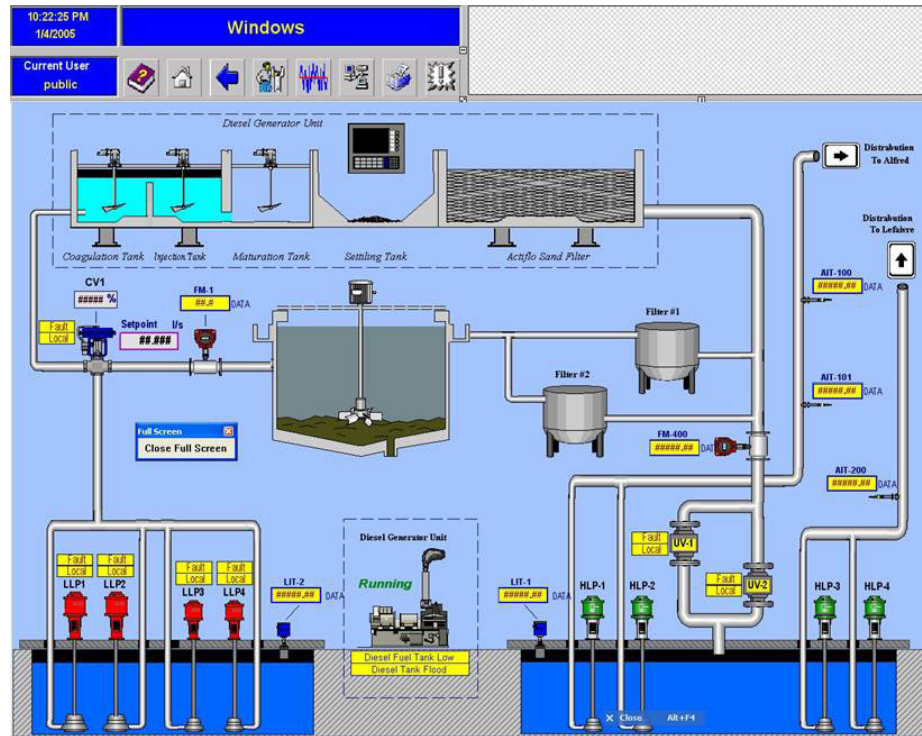
SAMPLE SCADA SYSTEMS
